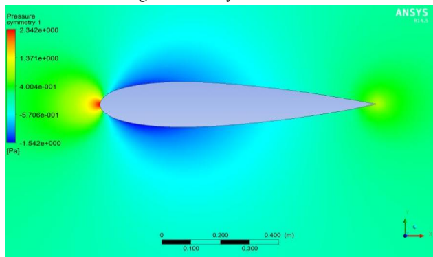
Fig 10: Pressure Distribution
